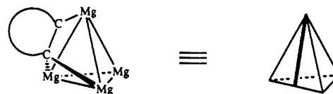
Figure 8. Schematic representation of a divalent organic group on top of one face of a tetrahedron of magnesium atoms.
